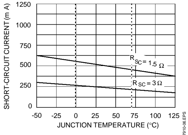
SHORT-CIRCUIT CURRENT
